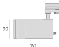
ZOOR LED spot II 30W
